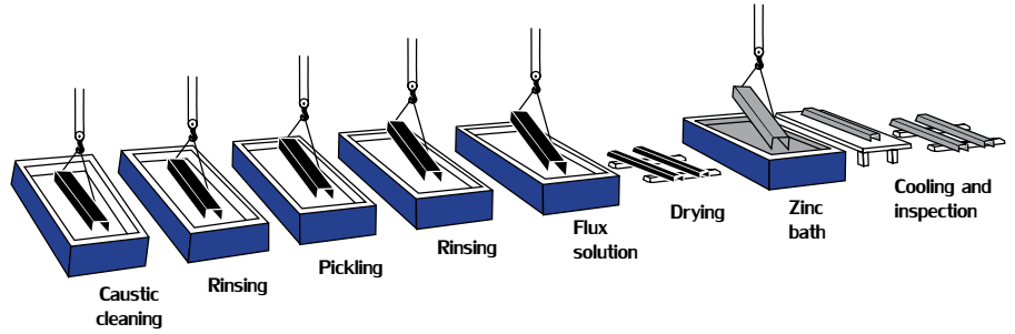
..... Figure 3: Batch Hot-Dip Galvanizing Process
