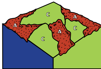
Mosaic of anodes and cathodes, electrically connected by the underlying steel.
